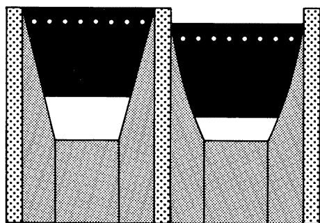
Belt should ride like this
