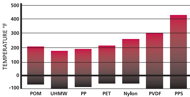
Fig 3: Continuous operation
